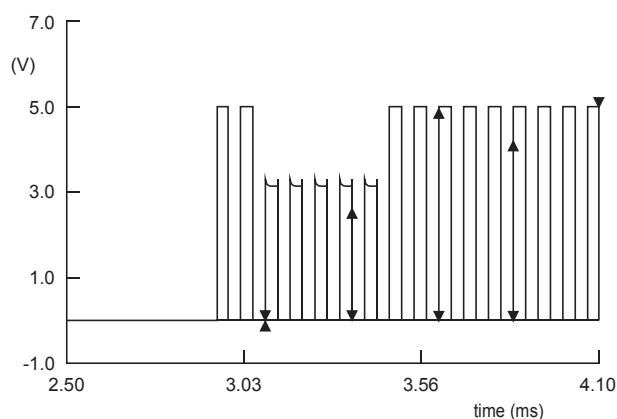
Fig 26. Example 1: overshoot_t1 = 2d; overshoot_t2 = 5d.
