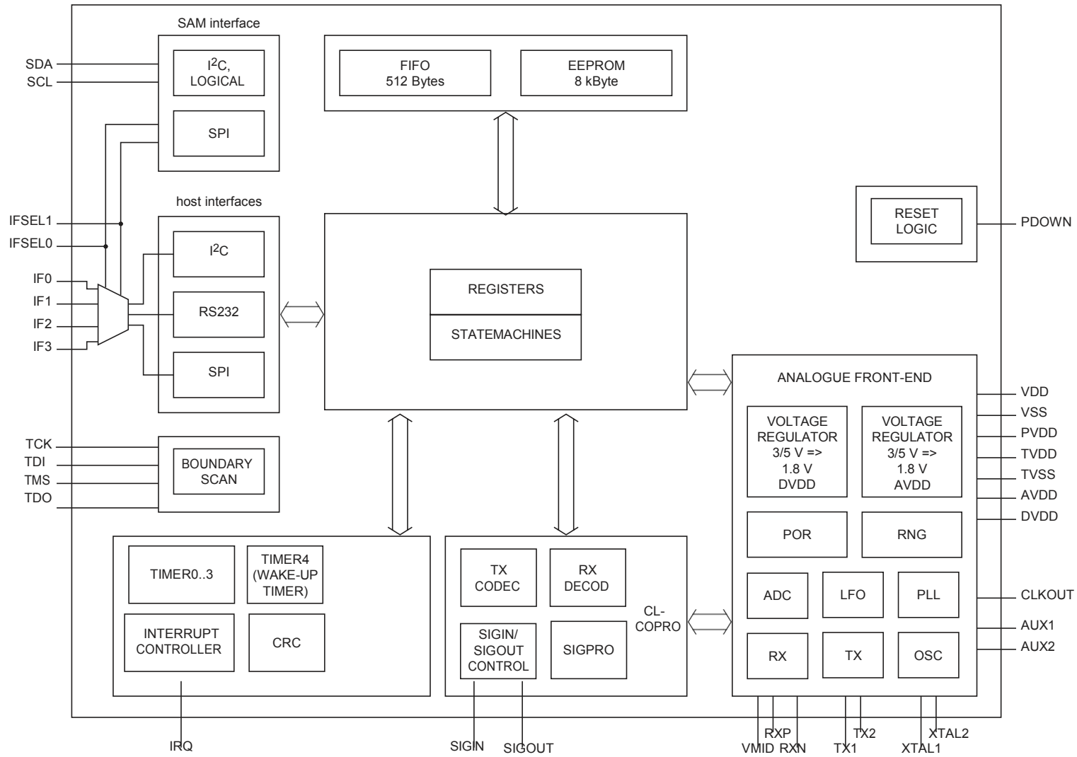
Fig 3. Detailed block diagram of the GDS9663
