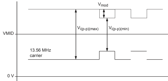
Fig 34. Pin RX input voltage
