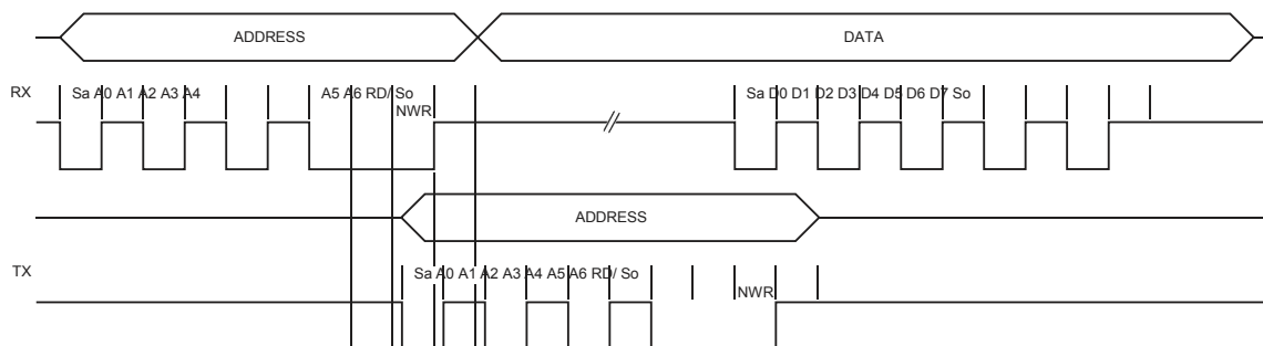
Fig 15. Timing diagram for UART write data
